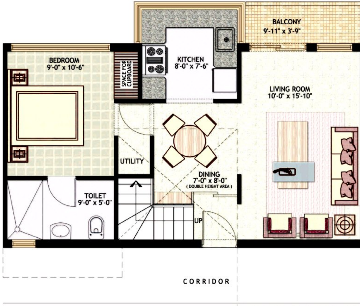
LOWER LEVEL PLAN
