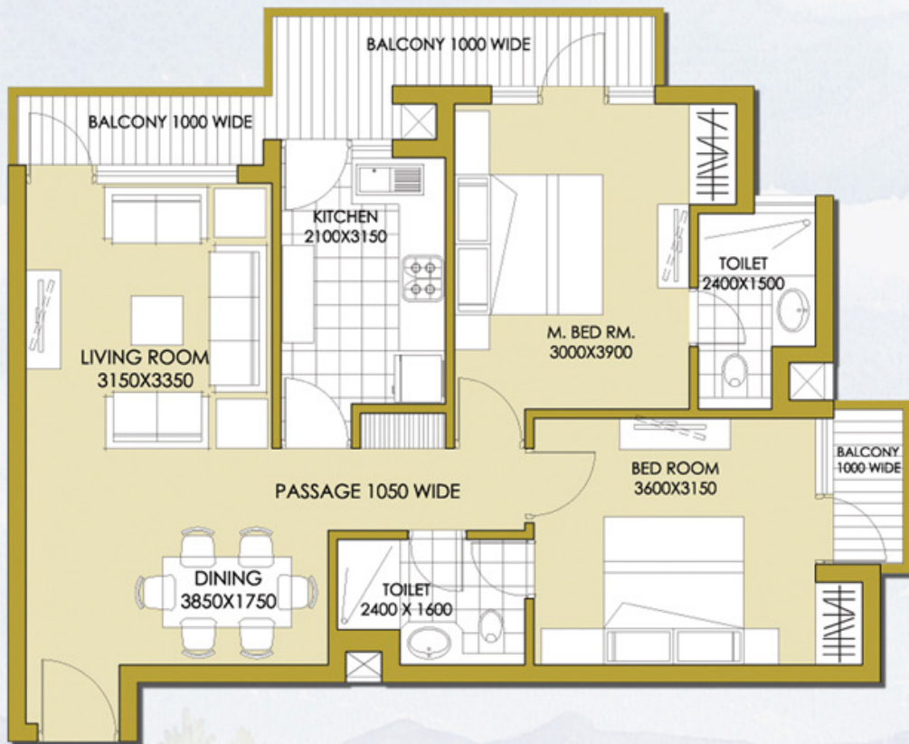
Typical 2Bhk unit (1100 sqft.)
